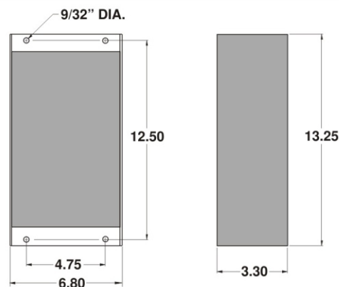
091-200-12 Outline Drawing
