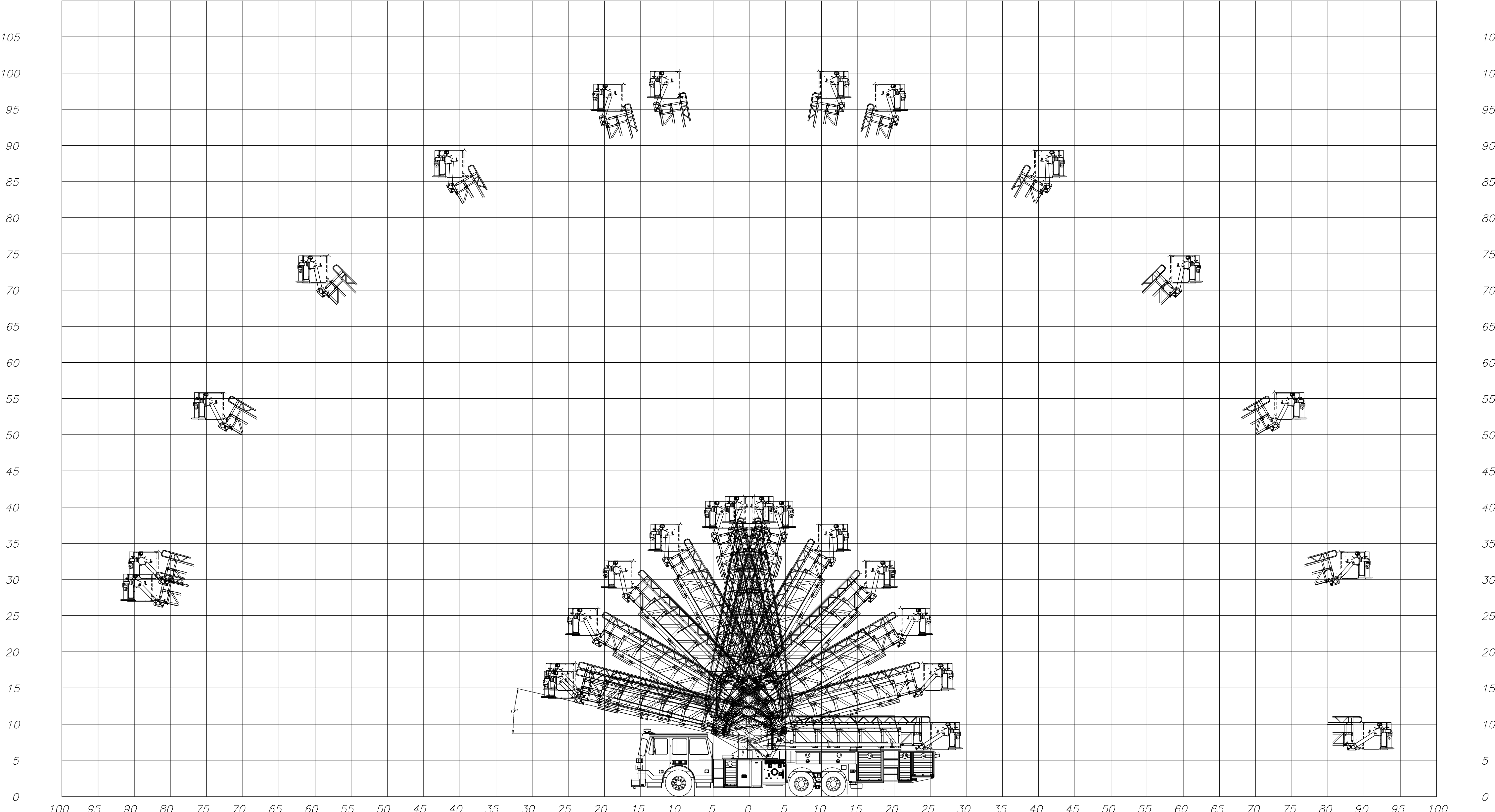
SUTPHEN 100' SPH PLATFORM 230"WB FLAT ROOF
