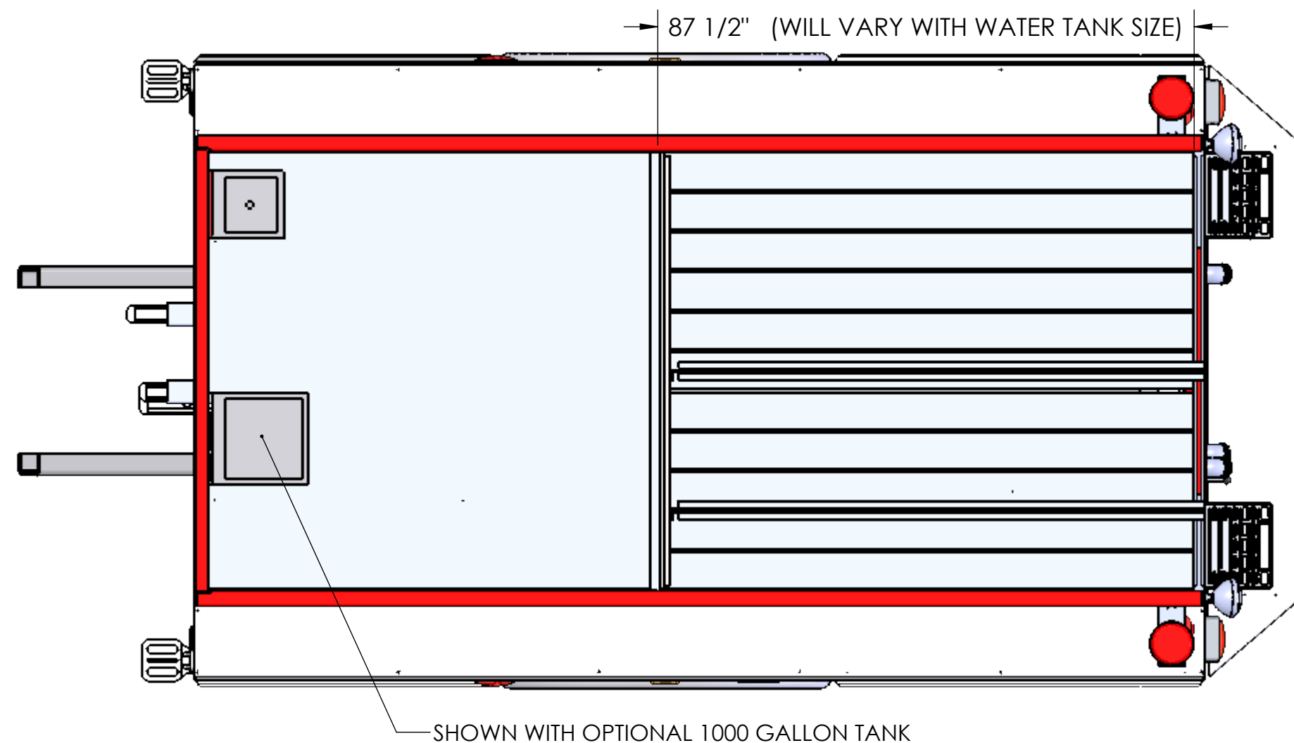
SHOWN WITH OPTIONAL 1000 GALLON TANK
