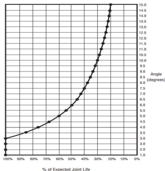
Joint Life vs. Joint Angle
