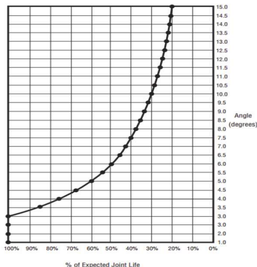
Joint Life vs. Joint Angle
