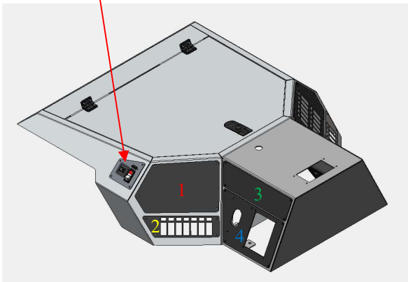
Lower Command Console (15L engine):
